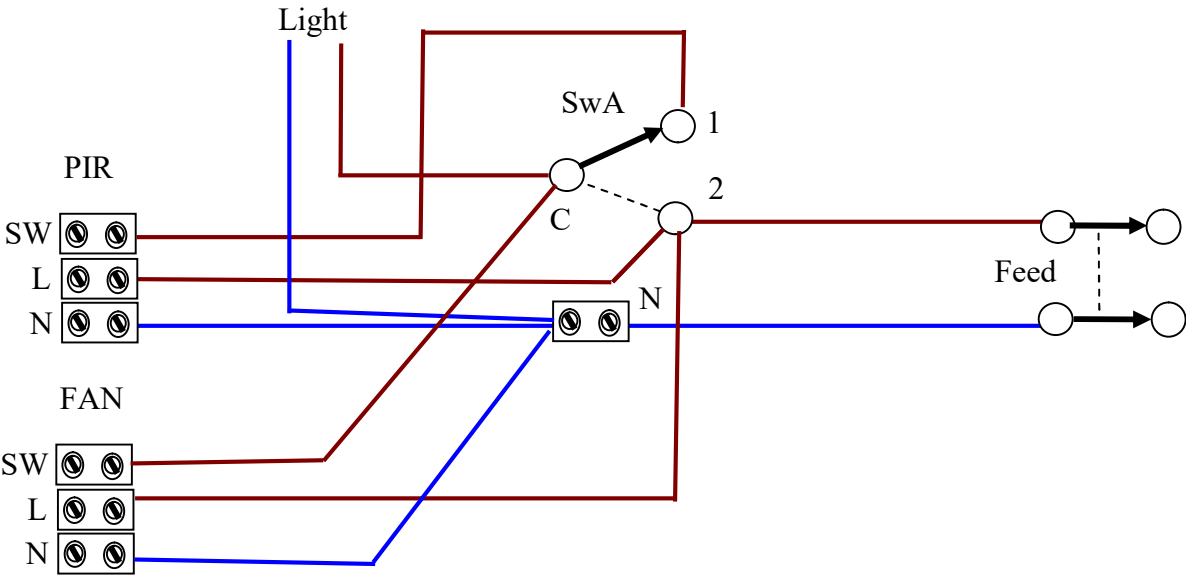
Light and Fan controlled with PIR Detector, Override switch and Isolator
